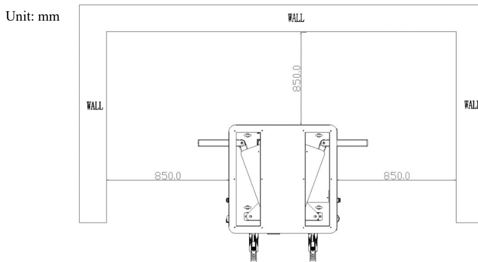
Figure 3 Charger maintenance distance diagram
