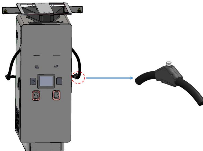
Figure 14 Position of the charging cable clamp
