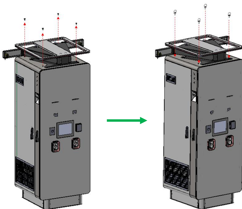
Figure 7 Removing top screws and installing lifting bolts
