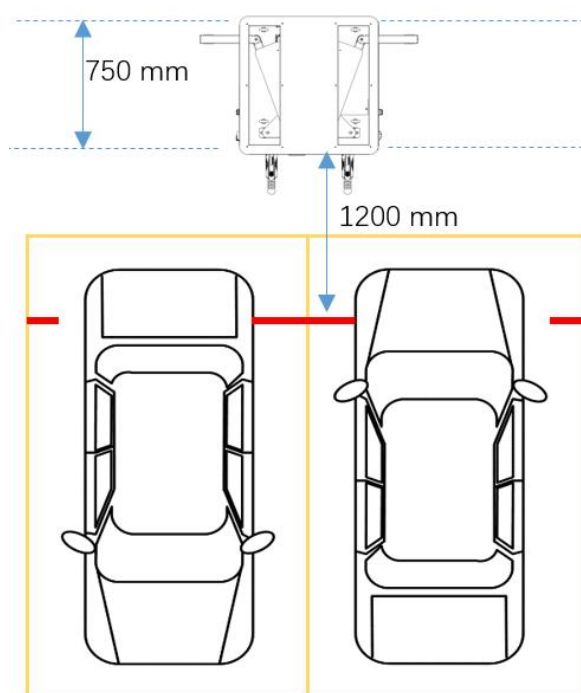
Figure 4 Requirement for parking spaces
