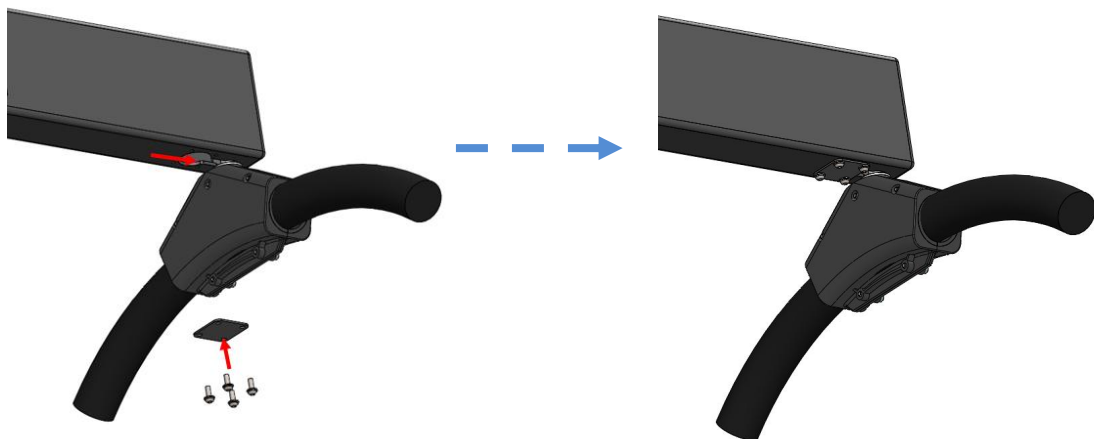
Figure 17 Fixing the charging cable clamp
