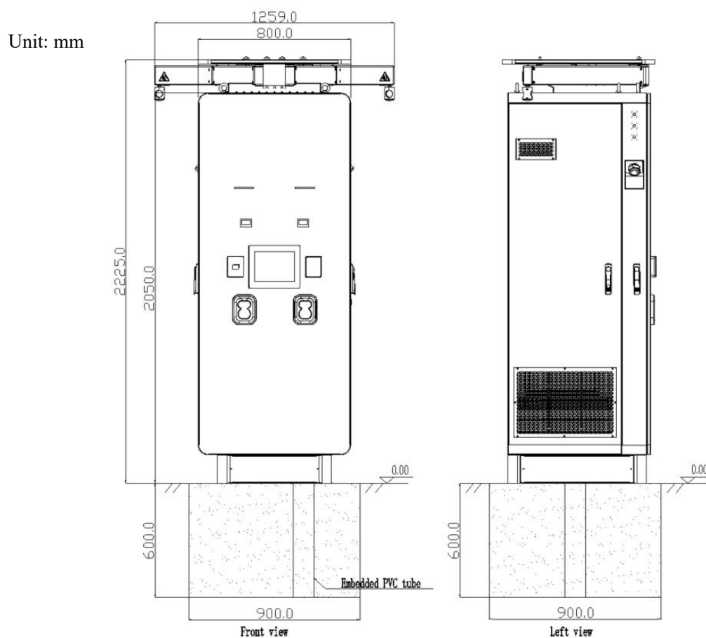
Figure 2 Front and left views of installation and construction
