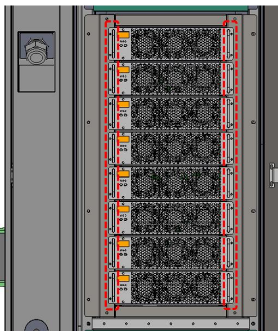
Figure 13 Installation position of power module screw
